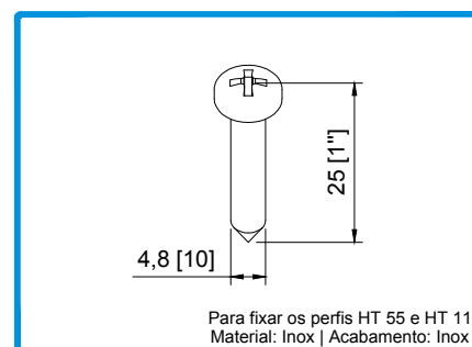
290171 PARAFUSO CQ 1x10 INOX
